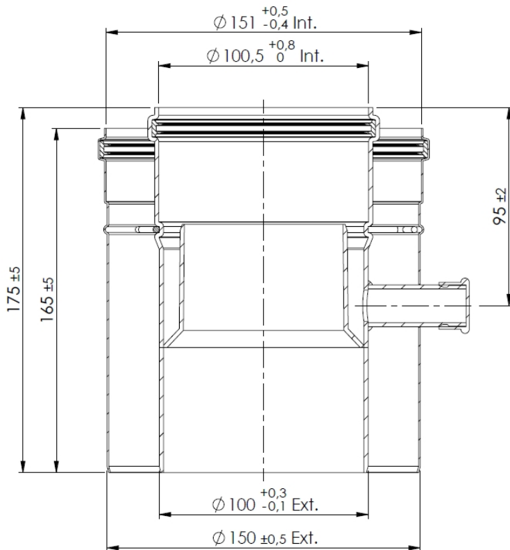
SECTION A-A Unit of measure: mm
